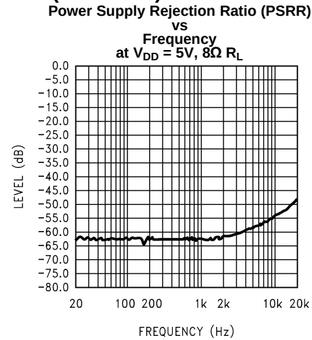
Figure 10. Input Floating
